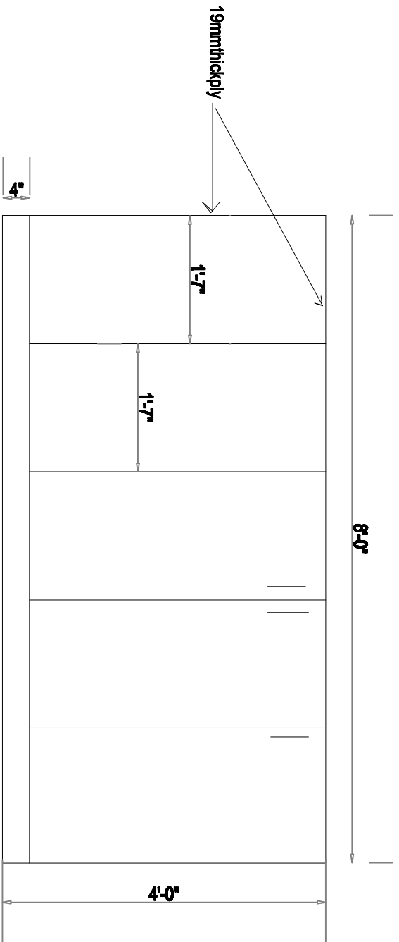
storage unit front elevation
